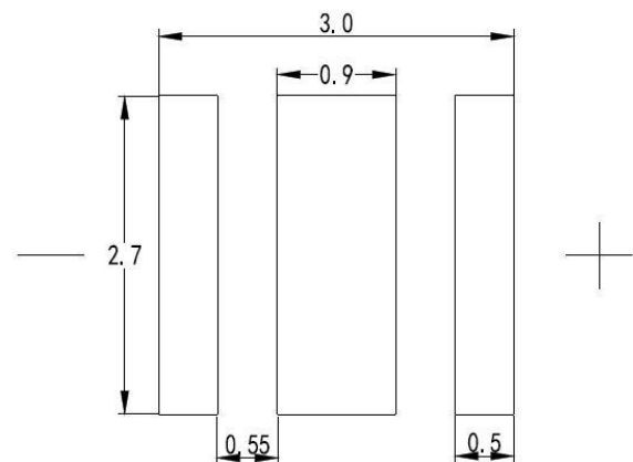
Recommended stencil
